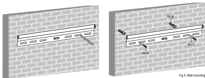
Fig. 6: Wall mounting
