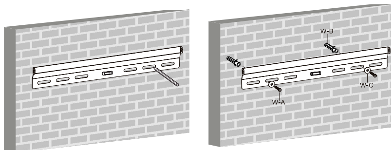
Fig. 10: Montage mural
