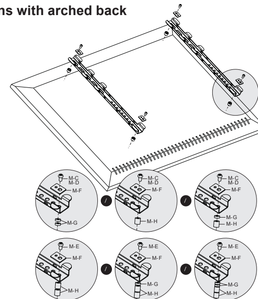
Fig. 8: Flat screens with arched back
