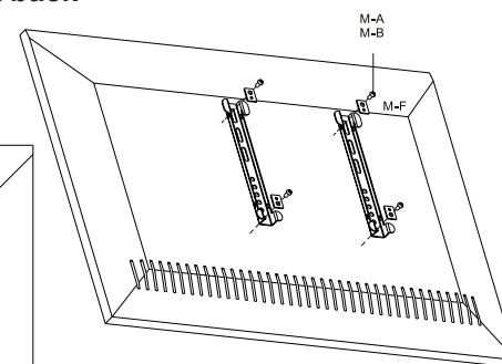
Fig. 7: Flat screens with flat back
