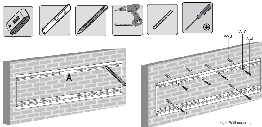
Fig. 8: Wall mounting
