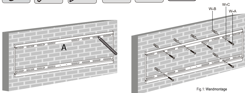
Fig. 1: Wandmontage
