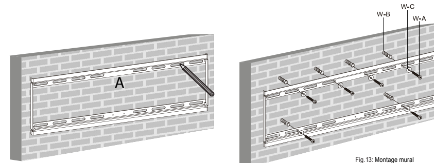
Fig. 13: Montage mural
