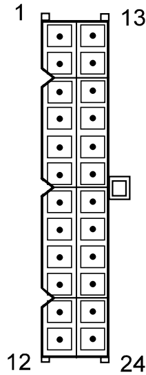
ATX 1.0 -plug 24 contacts
